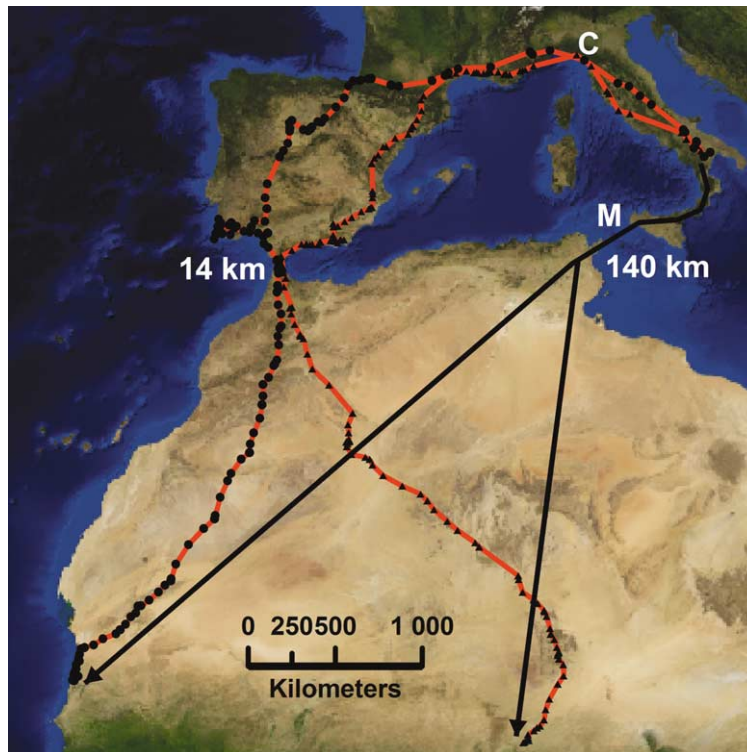
Figure 1. Autumn migratory routes of two juvenile short-toed eagles born in southern Italy and tracked by satellite telemetry (Biagio: circles; Nic: triangles). The tracks interpolations of the GPS locations (see Methods). Black tracks: direct, hypothetic, routes across the Sicily Channel. The over-water distances (km) of the two possible sites to cross the Mediterranean Sea (Gibraltar: 14 km; Sicily: 140 km) are indicated. 'C' (Capriglia) and 'M' Marettimo are the watchsites where the field observations mentioned in the discussion have been carried out.
