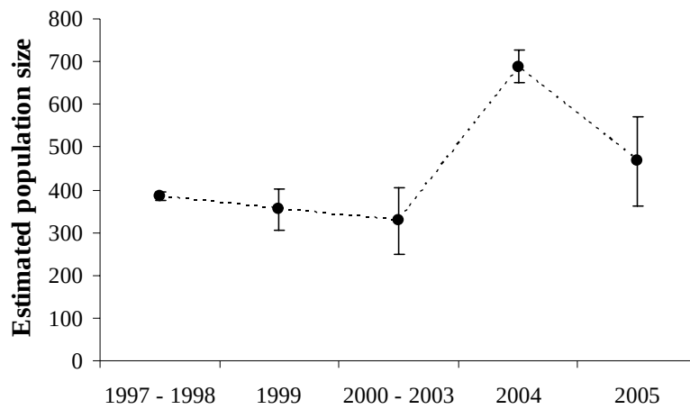
FIGURE A3-1d). Estimates of population size during the study periods at colony HO (Hormigas).
